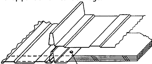
#10 - 12 X 1" Type A Pancake Head Wood Screw at 10 3/8" Centers
